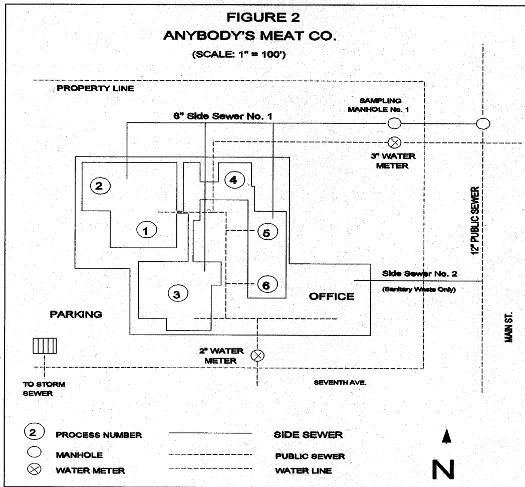
FIGURE 2. BUILDING LAYOUT
